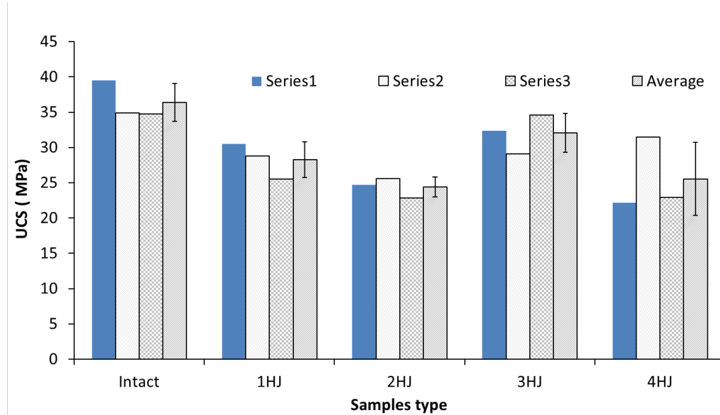
FIGURE 5. UCS versus samples type
