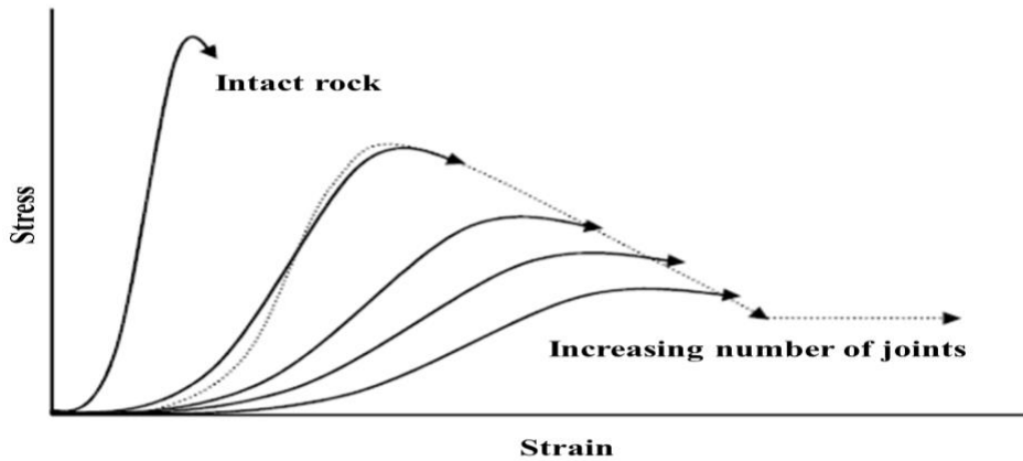
FIGURE 1. Stress–strain behaviour of rock mass with increasing joints [9]
