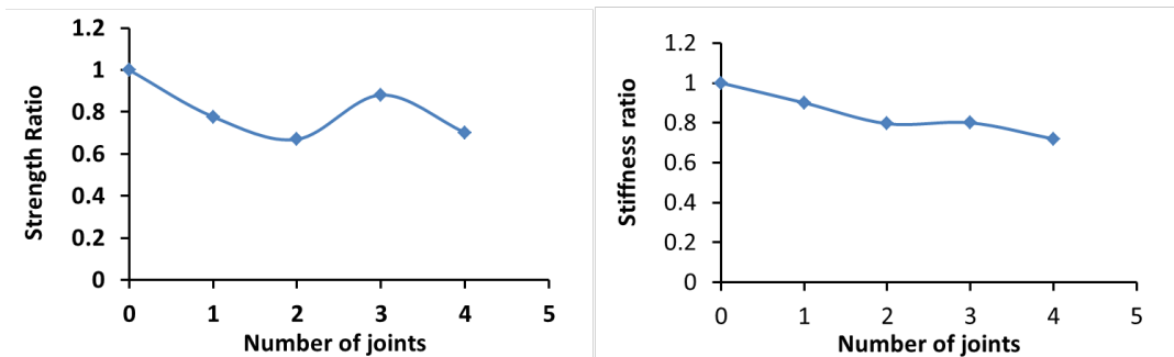
FIGURE 8. (left) strength ratio versus number of joints; (right) stiffness ratio versus number of joints
