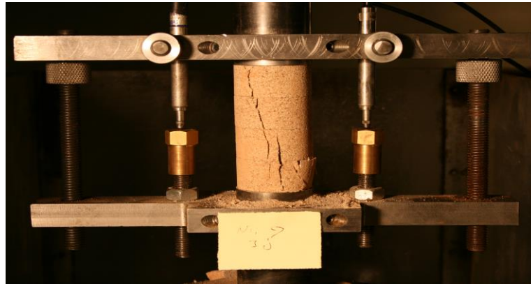
FIGURE 3. Sample within UCS test apparatus showing LVDTs.
